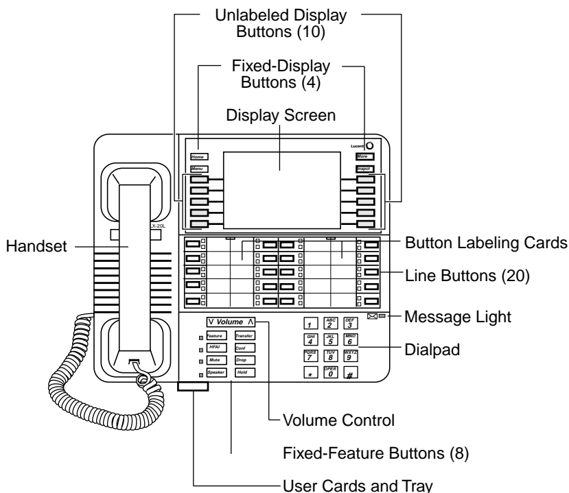
Figure 3-5. MLX-20L Telephone
