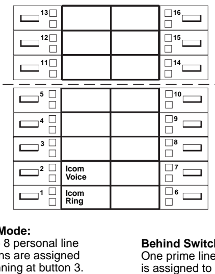
Figure G-6. MLX-16DP Telephone (Key and Behind Switch Modes)
