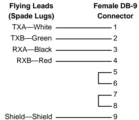
CAB-108 (2-ft. [0.6 m])
