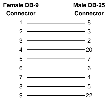
9-Pin to 25-Pin Serial Cable
