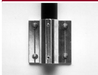
No. 52E Extruded HD Wall Flange (4-Hole)
