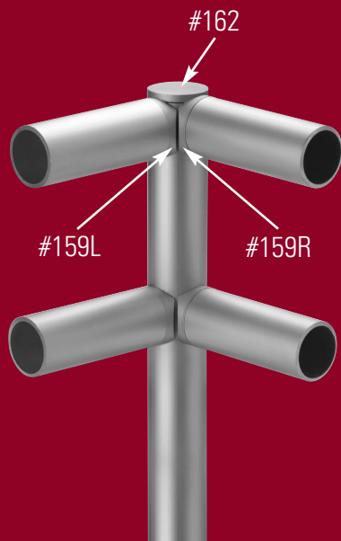
Typical Corner Post Assembly
