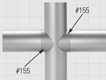
Typical Assembled Cross
