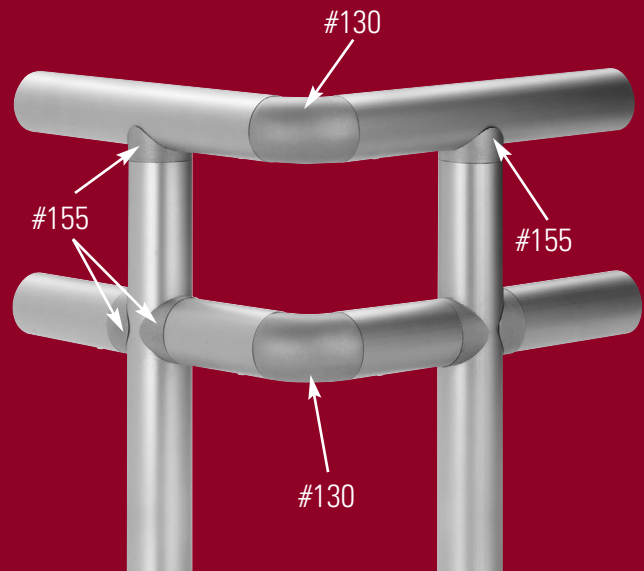
Corner Elbow Assembly
